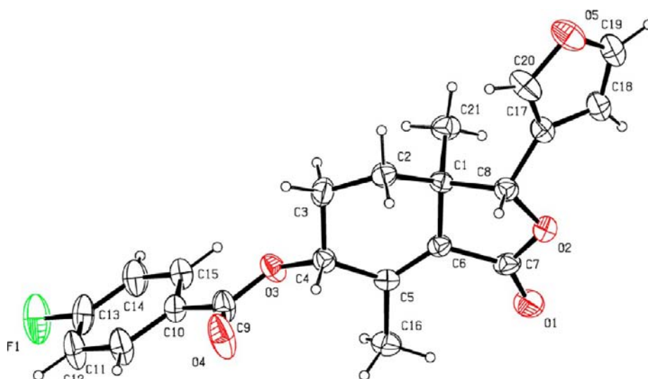
Figure 2. X-ray crystal structure of 6h .
