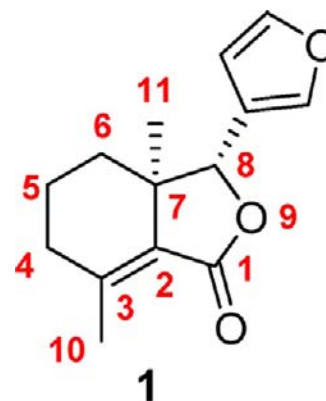
Figure 1. Chemical structure of fraxinellone ( 1 ).
